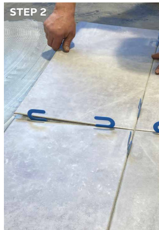
STEP 2 And now apply the tiles using spacers within the next 30 minutes. Take the spacers out within 45-60 minutes and roll the floor.
